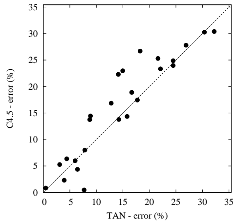
Figure 6. Error curves comparing smoothed TAN (solid, x axis) with C4.5 (dashed, y axis). In the error curves, the smaller the value, the better the accuracy. In the scatter plot, points above the diagonal line correspond to datasets where smoothed TAN performs better, and points below the diagonal line correspond to dataset where C4.5 performs better. See the caption of Figure 2 for a more detailed description.
