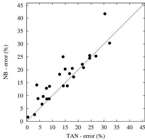
Figure 4. Error curves comparing smoothed TAN (solid, x axis) with naive Bayes (dashed, y axis). In the error curves, the smaller the value, the better the accuracy. In the scatter plot, points above the diagonal line correspond to datasets where smoothed TAN performs better, and points below the diagonal line correspond to datasets where naive Bayes performs better. See the caption of Figure 2 for a more detailed description.
