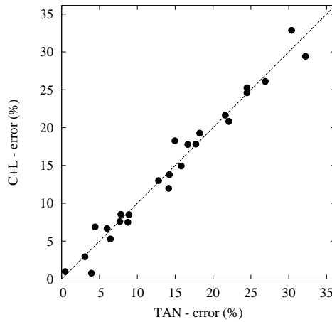
Figure 7. Error curves comparing smoothed TAN (solid line, x axis) with smoothed Chow and Liu's classifier (dashed line, y axis). In the error curves, the smaller the value, the better the accuracy. In the scatter plot, points above the diagonal line corresponds to datasets where smoothed TAN performs better and points below the diagonal line corresponds to datasets where smoothed Chow's and Liu's classifier performs better. See the caption of Figure 2 for a more detailed description.
