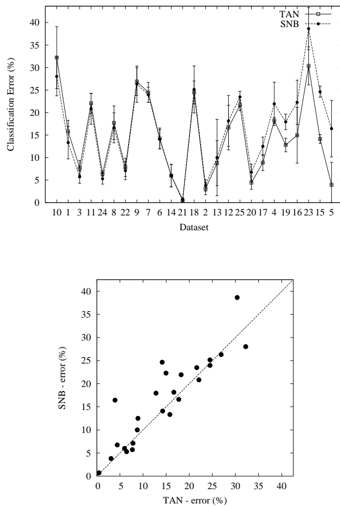
Figure 5. Error curves comparing smoothed TAN (solid, x axis) with selective naive Bayes (dashed, y axis). In the error curves, the smaller the value, the better the accuracy. In the scatter plot, points above the diagonal line correspond to datasets where smoothed TAN performs better, and points below the diagonal line correspond to datasets where selective naive Bayes performs better. See the caption of Figure 2 for a more detailed description.
